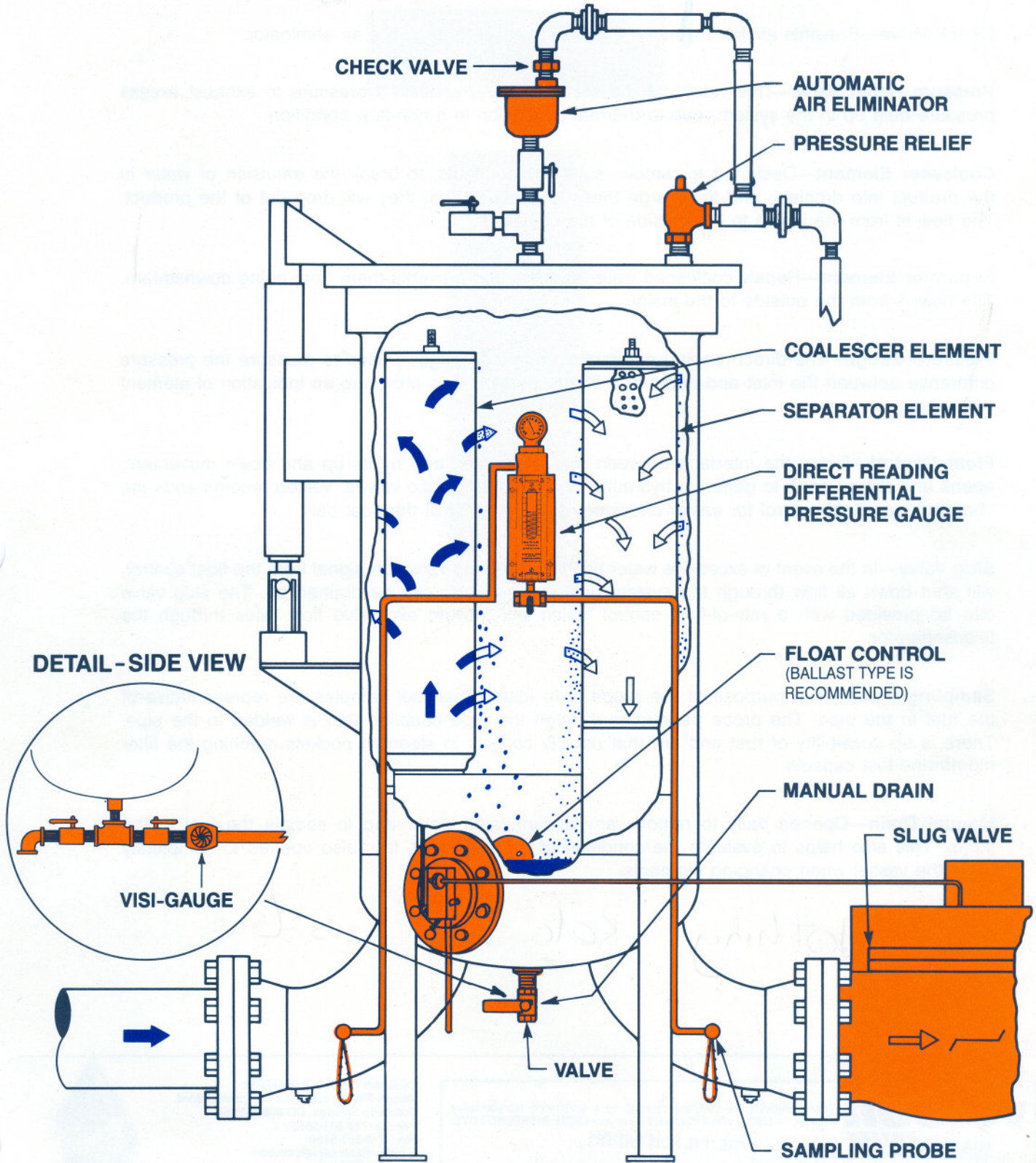
CUTAWAY—TYPICAL FILTER SEPARATOR
